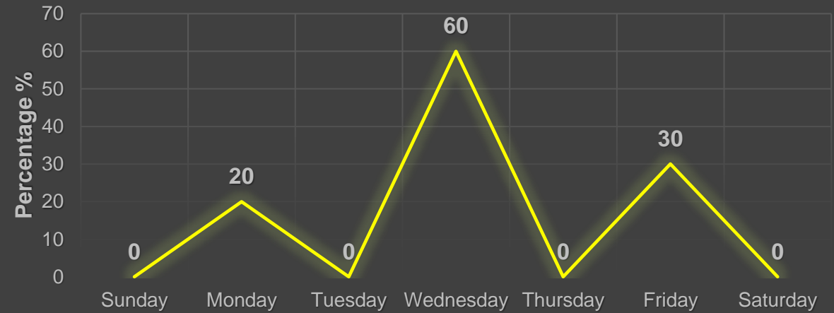
Precipitation
