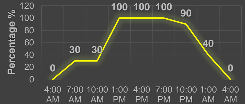
Precipitation
