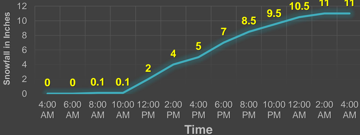
Snowfall Amount
